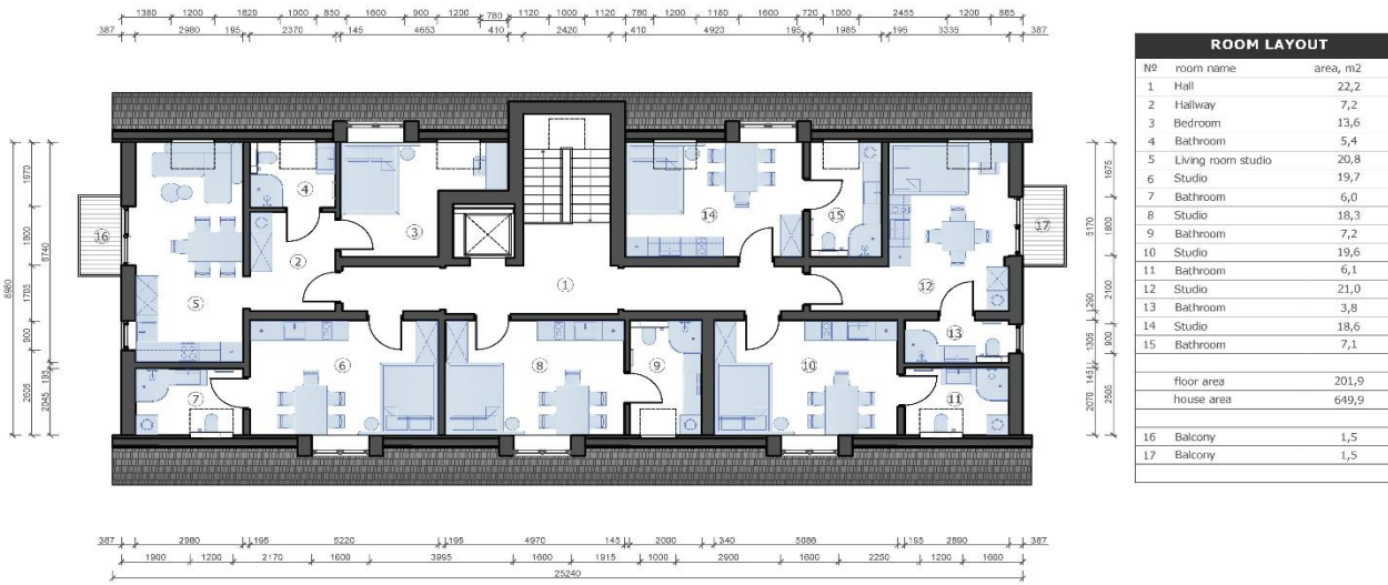
3 floor plan. 1:100 (A-3)
